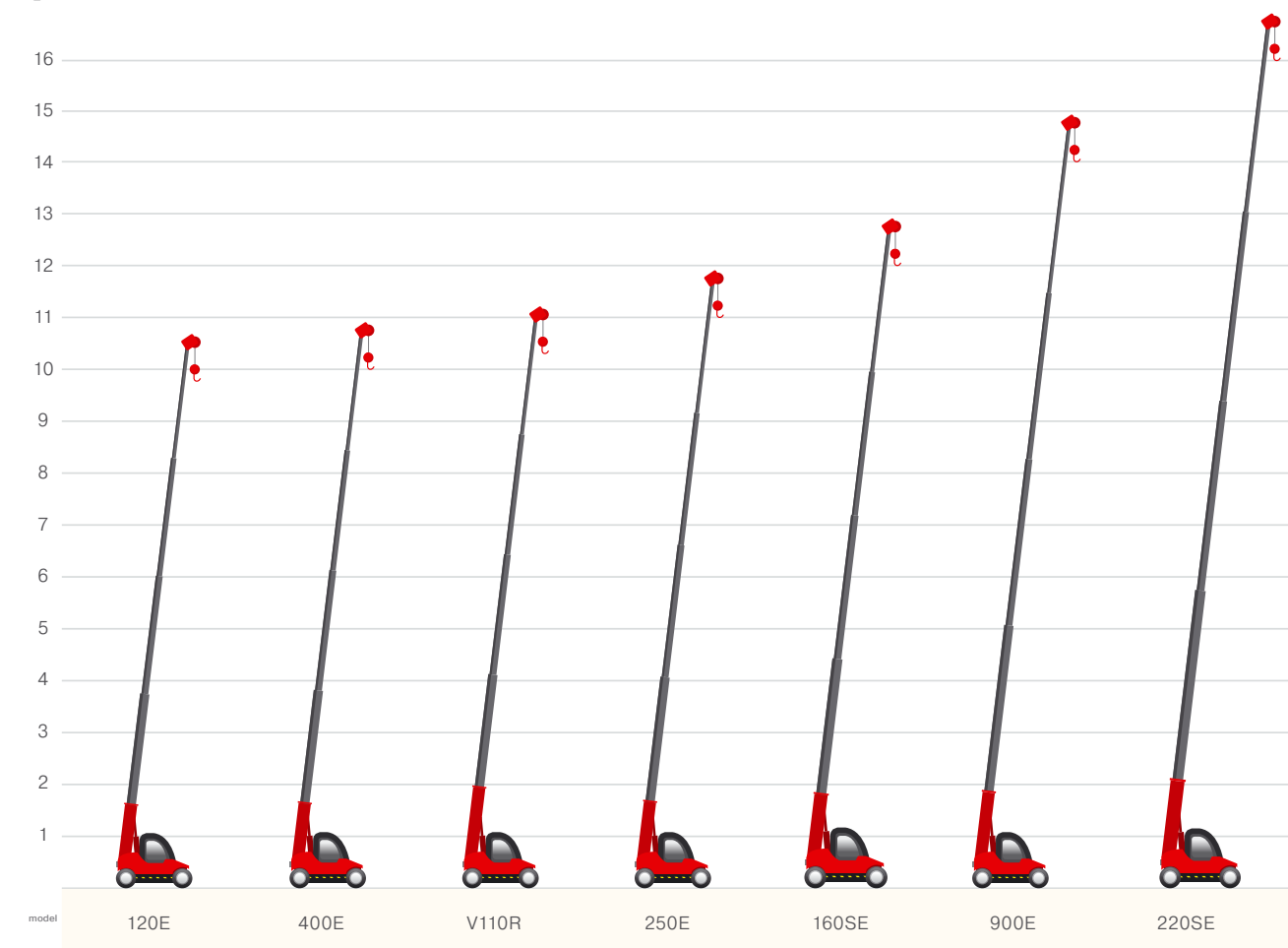
■ Hook lifting height of Valla industrial crane, electric drive.
