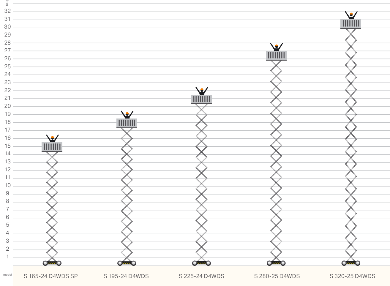
Working height of H.A.B. scissor lifts, diesel power drive.
