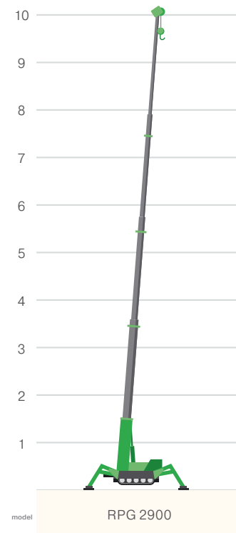
Hook lifting height of Palcrane RPG 2900
