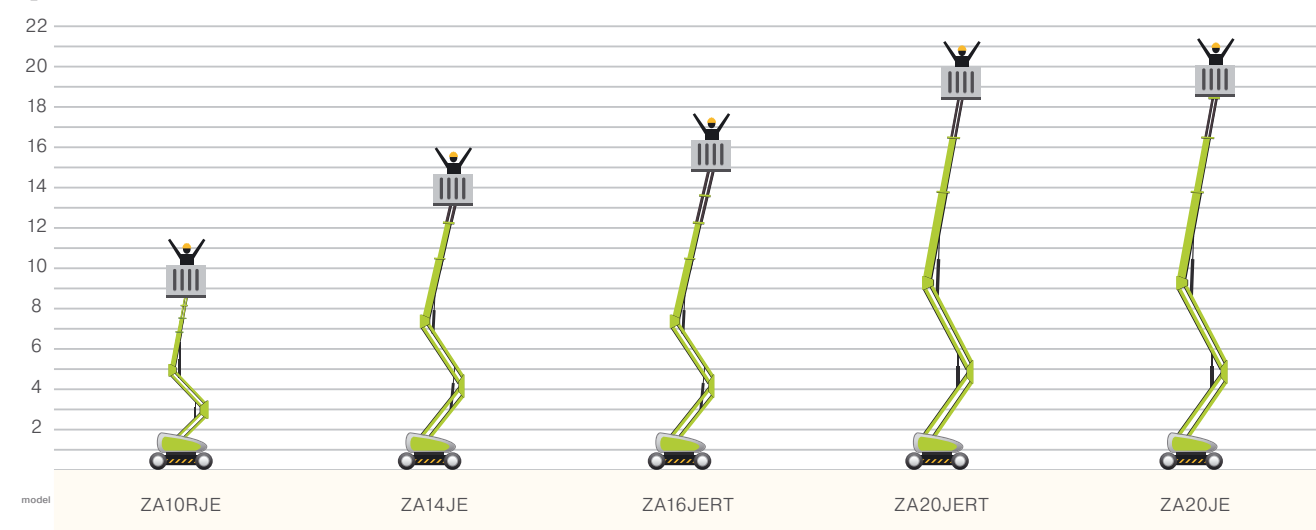
Working height of Zoomlion articulating boom lifts, electric drive.
