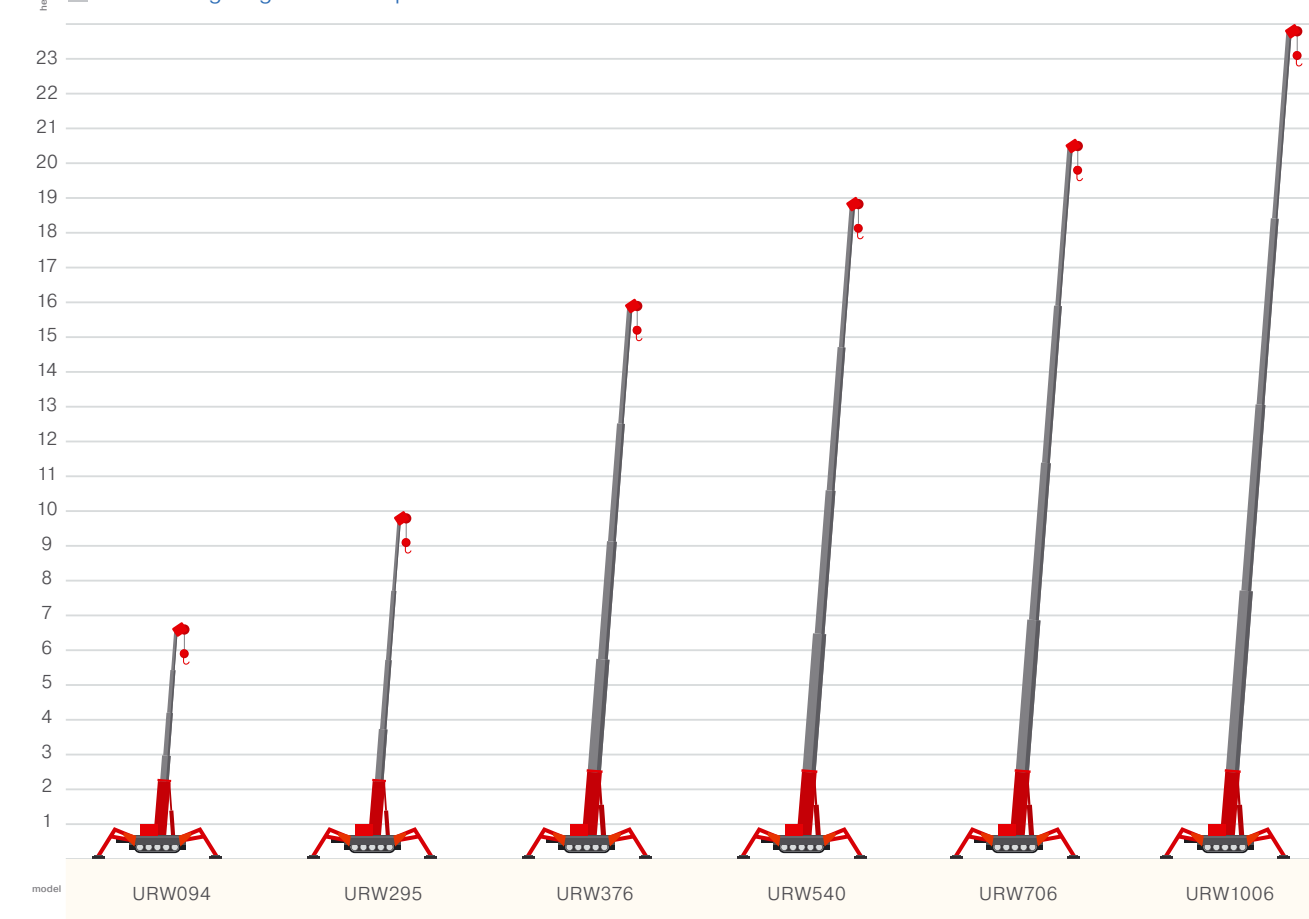
Hook lifting height of UNIC spider cranes.
