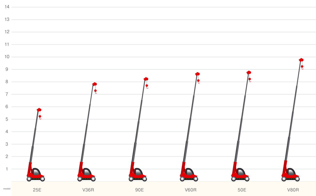
■ Hook lifting height of Valla industrial crane, electric drive.
