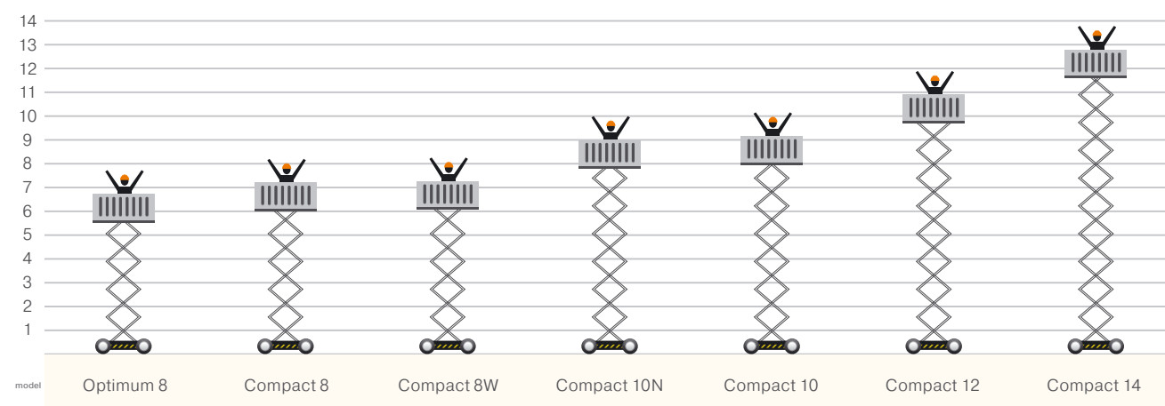
Working height of Haulotte scissor lifts, electric drive.
