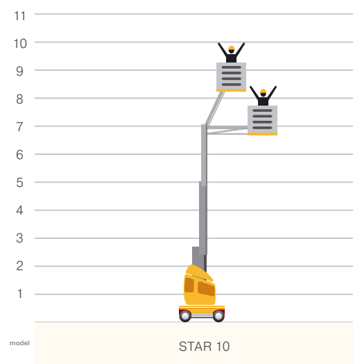
Working height of Haulotte vertical lifts with a jib, electric drive.
