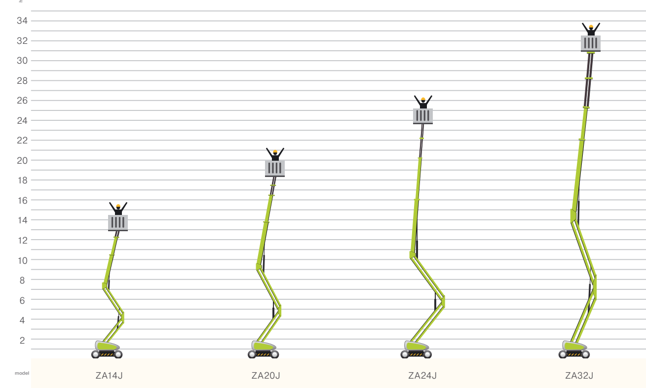
Working height of Zoomlion articulating boom lifts, diesel power drive.
