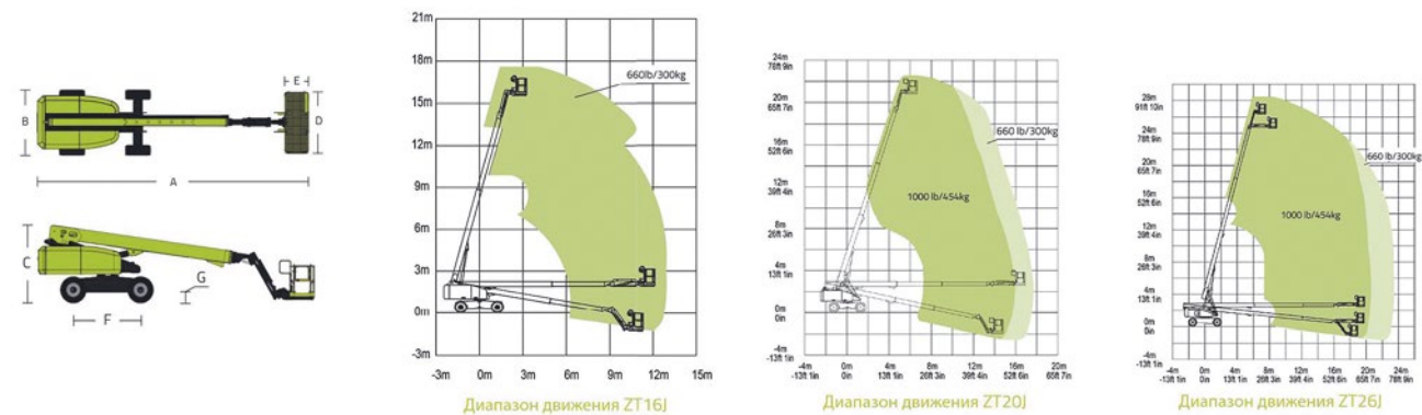
Working height of Zoomlion telescopic lifts, diesel power drive.
