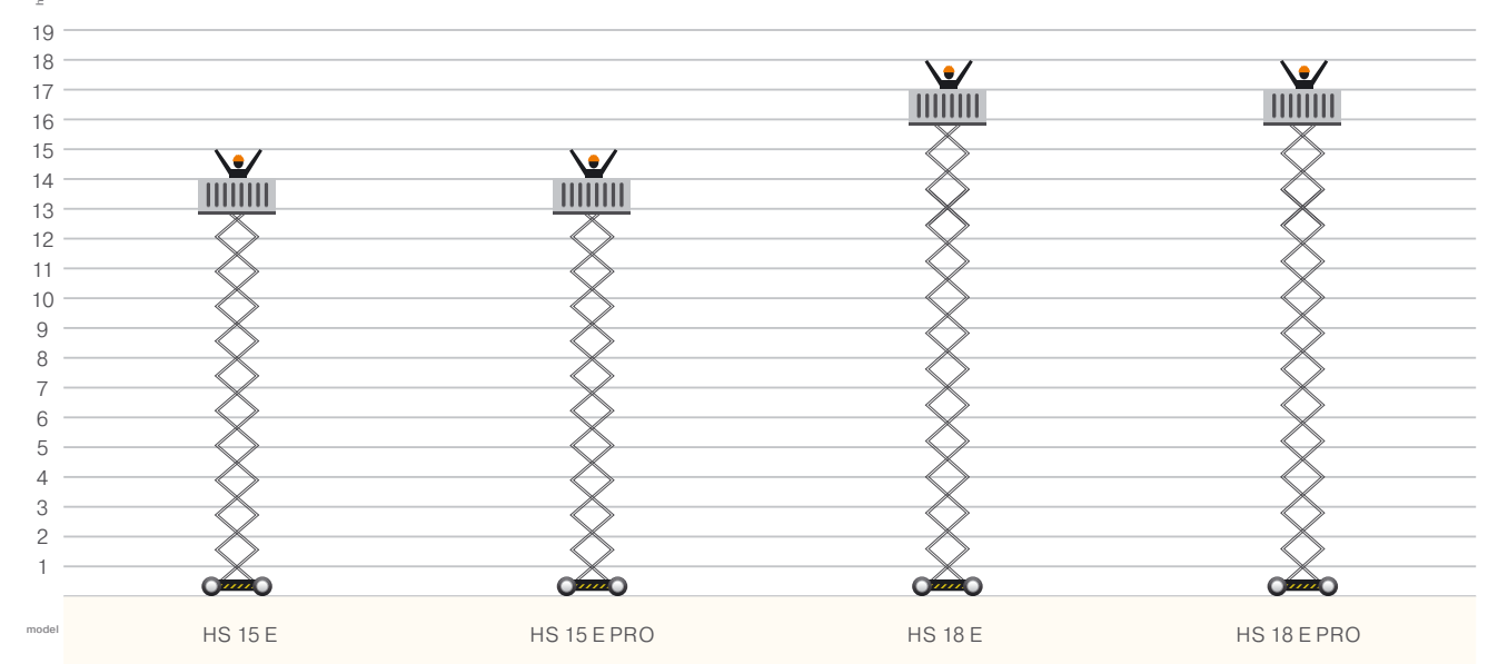
Working height of Haulotte rough terrain scissor lifts, electric drive.
