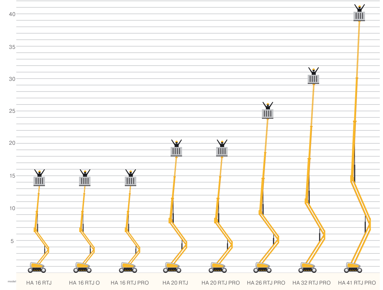
Working height of Haulotte articulating boom lifts, diesel power drive.
