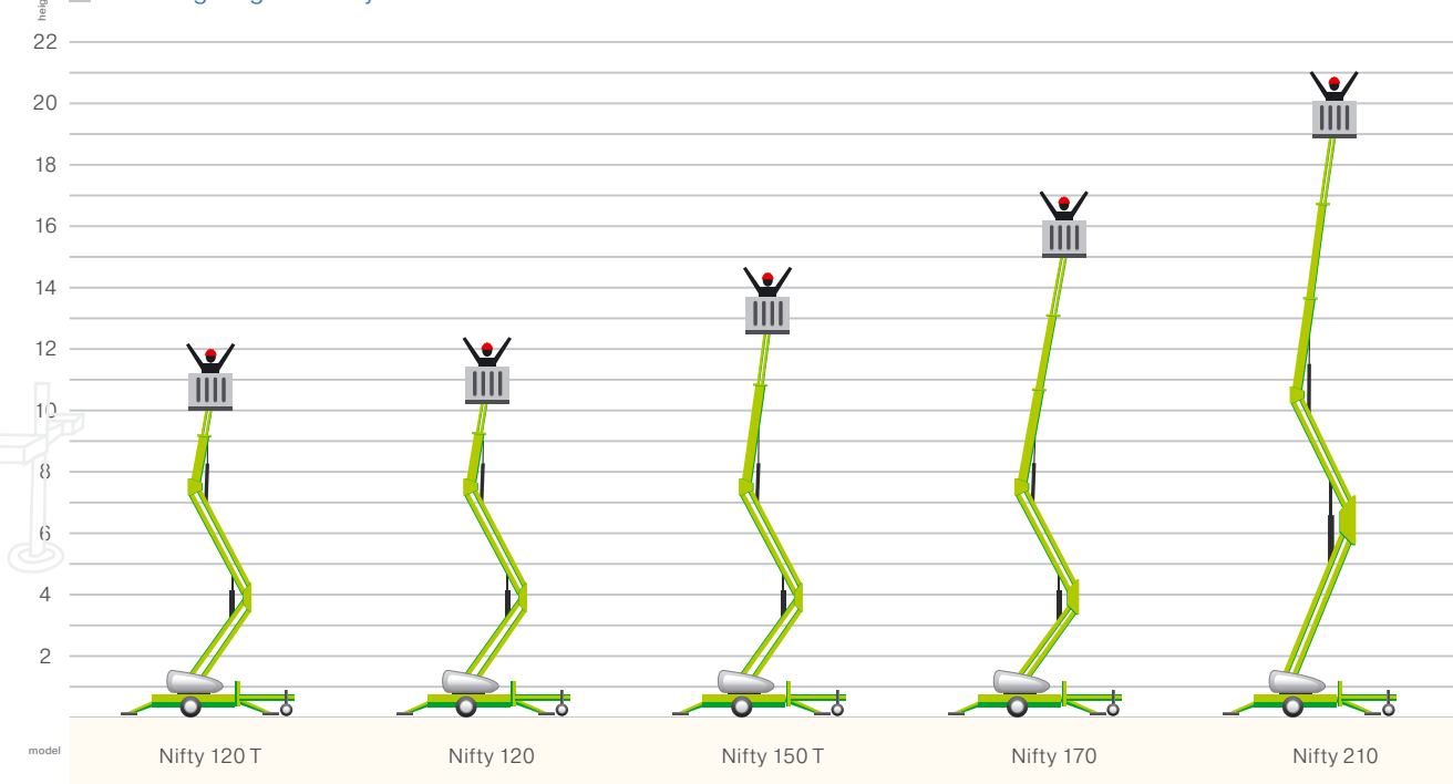
Working height of NiftyLift trailer-mounted lifts
