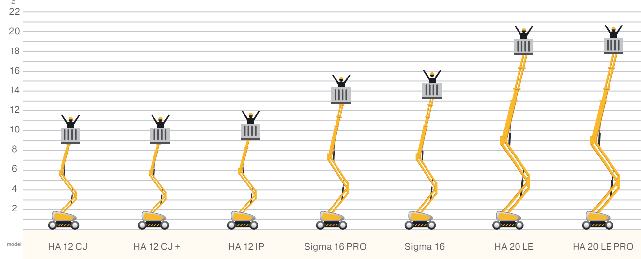
Working height of Haulotte articulating boom lifts, electric drive.
