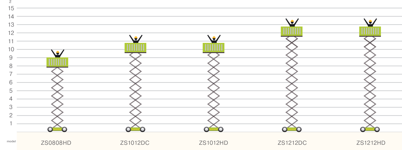
■ Working height of Zoomlion scissor lifts, electric drive.
