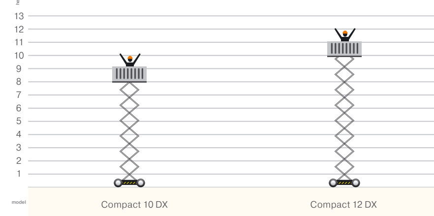
Working height of Haulotte scissor lifts, diesel power drive.
